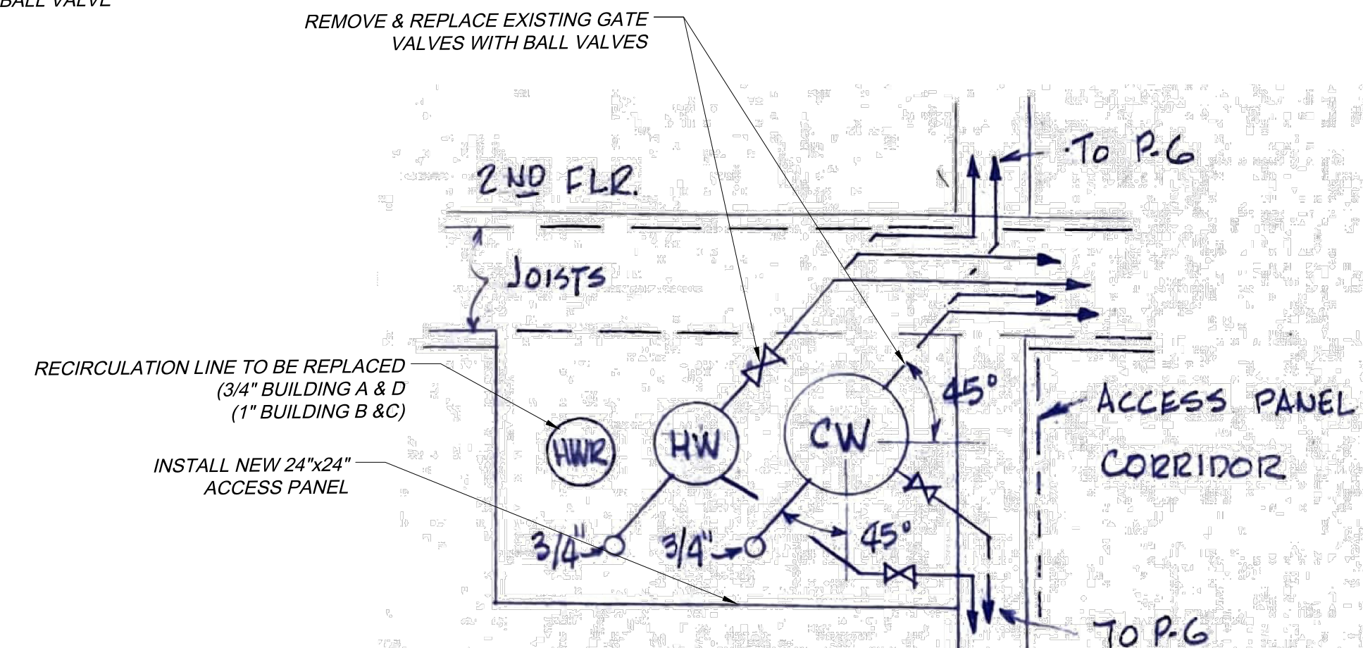
WATER LINE DETAIL NOT TO SCALE
